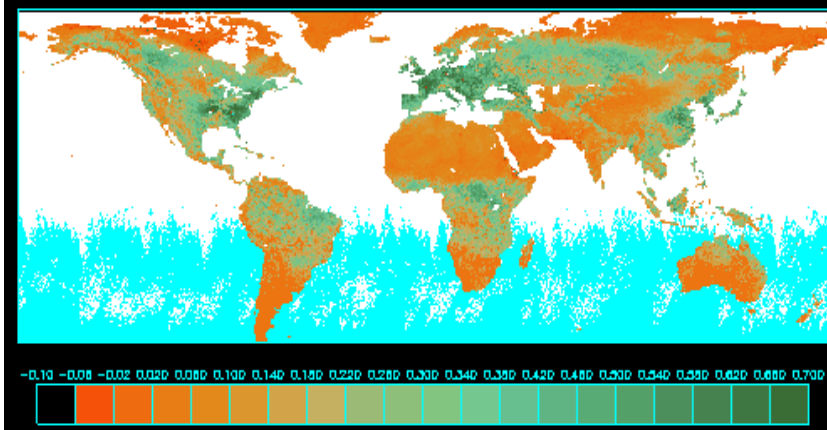
GVI Normalized Difference Vegetation Index: MAY 17 2015
