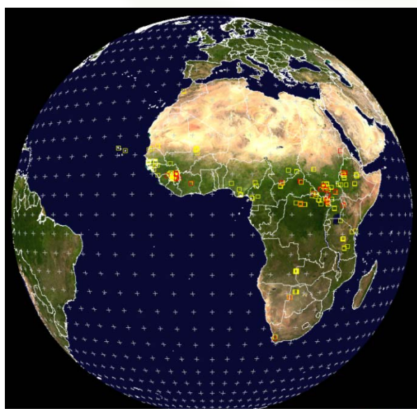
MPEF FIRE 2015-02-23 12:00 UTC Legend: Yellow square = Probability of Fire, Red square = High Probability of Fire EUMETSAT
