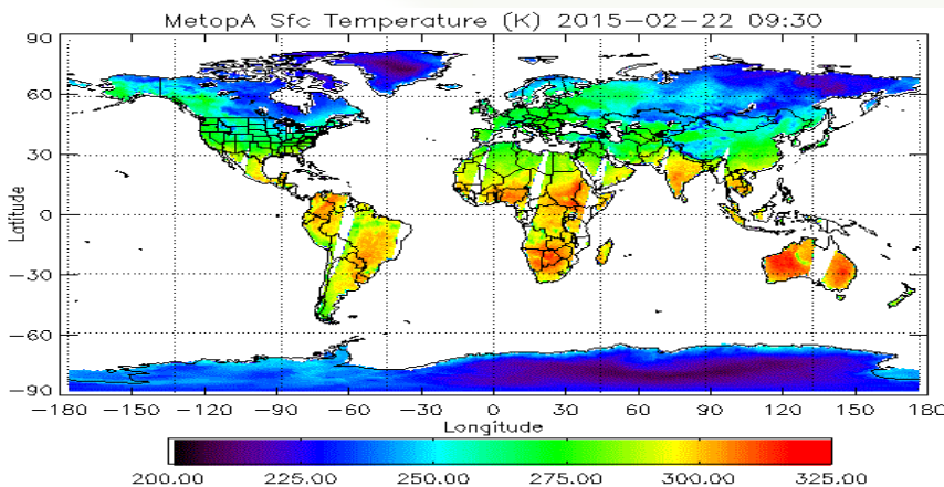
Sample image: Surface Temperature
