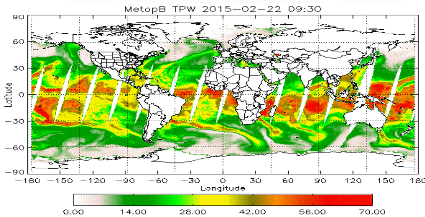
Sample image: Total Precipitable Water
