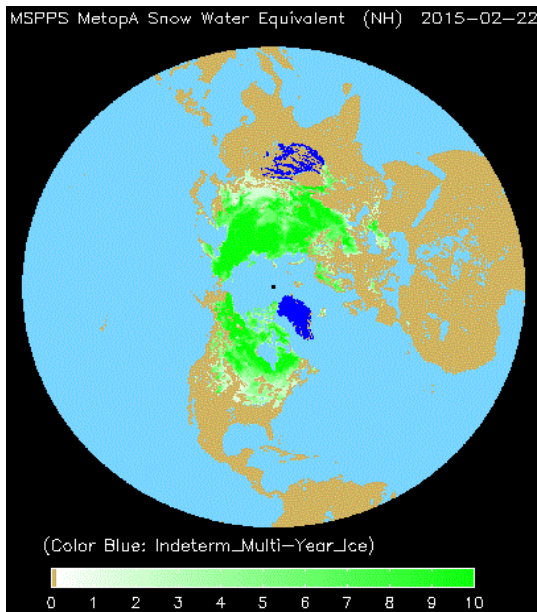
Sample image: Snow Water Equivalent
