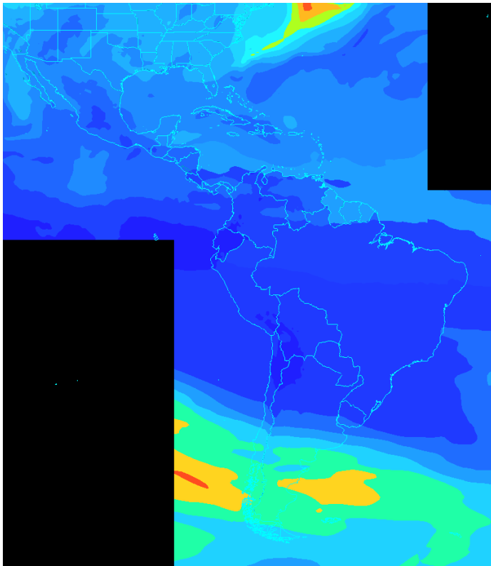
Sample image: Total ozone @ Entire atmosphere layer
